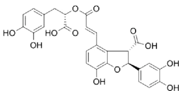
Lithospermic acid
